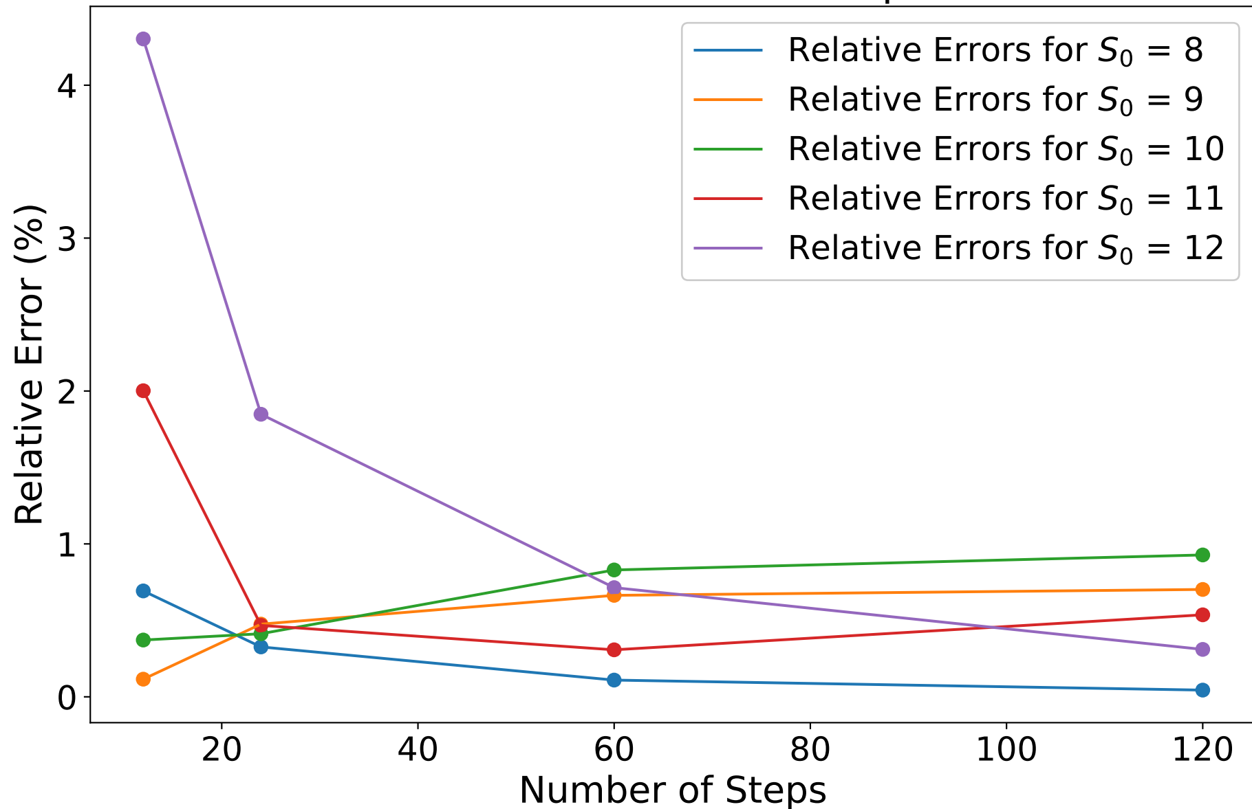
Relative Error of American Put Option Prices
